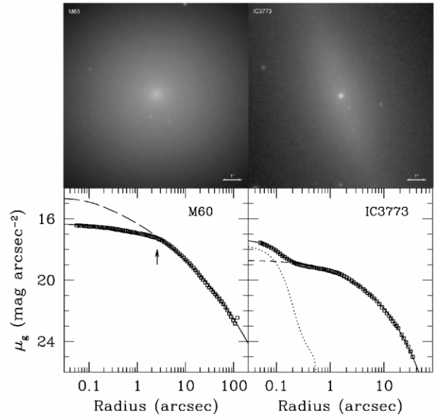
FIG. 1.—Upper panels: g -band images showing the central regions of M60 (left) and IC 3773 (right), the third and 51st brightest galaxies, respectively, in the ACSVCS. Lower panels: Azimuthally averaged g -band surface brightness profiles for the same two galaxies. M60 is a typical nonnucleated “core-Sérsic” galaxy: the best core-Sérsic model is shown as a solid curve. The vertical arrow shows the radius, r_b , at which the outer Sérsic profile “breaks” to an inner power law; the long-dashed curve shows the inward extrapolation of the Sérsic model fitted to the data beyond r_b . For IC 3773, we show the best-fit model that consists of a central King model for the nucleus (dotted curve) and a Sérsic model for the underlying galaxy (dashed curve). The solid curve shows the composite model.
