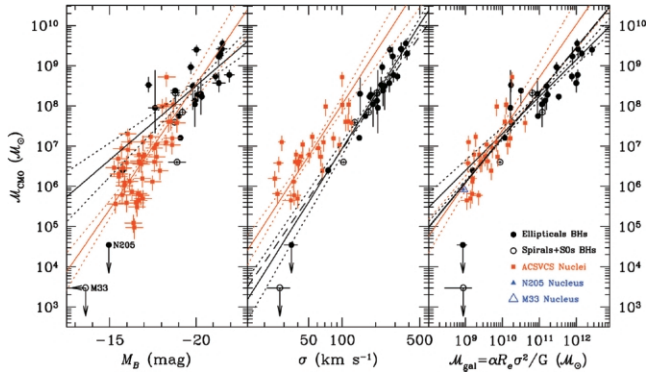
FIG. 2.— Left panel: Mass of the CMO plotted against absolute blue magnitude of the host galaxy (or bulge for spiral galaxies). Nuclei from the ACSVCS are shown as red squares. The SBHs in early-type and spiral galaxies are shown as filled and open circles, respectively. Middle panel: CMO mass as a function of the velocity dispersion of the host galaxy, measured within R_e . Right panel: CMO mass plotted against galaxy mass, defined as \mathcal{M}_{\text{gal}} \equiv \alpha R_e \sigma^2 / G with \alpha = 5 . In all panels, the solid red and black lines show the best fits to the nuclei and early-type SBH samples, respectively, with 1 \sigma confidence levels shown by the dotted lines. In the middle panel, the dashed line is the best-fit \mathcal{M}_{\text{SBH}}-\sigma relation of Tremaine et al. (2002). In the right panel, the dashed line is the fit obtained for the combined nuclei+SBH sample. Coefficients for all fits are listed in Table 1. For a larger version of this figure, please see the ACSVCS Web page http://www.cadc.hia.nrc.gc.ca/community/ACSVCS/publications.html .
